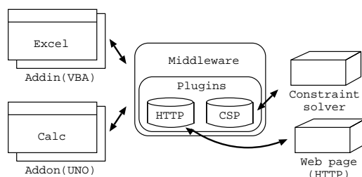
図 1: Architecture
