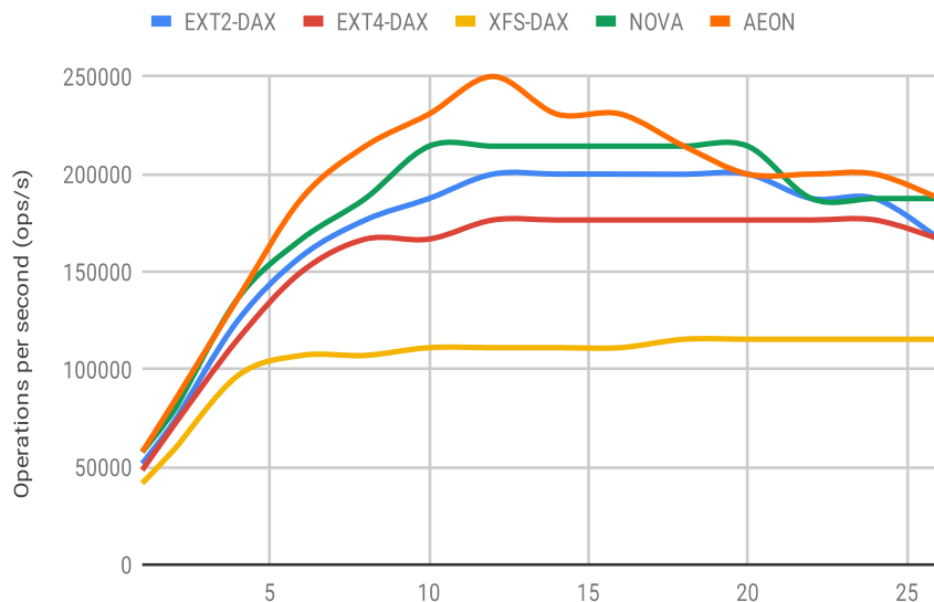
Create (more is better)
