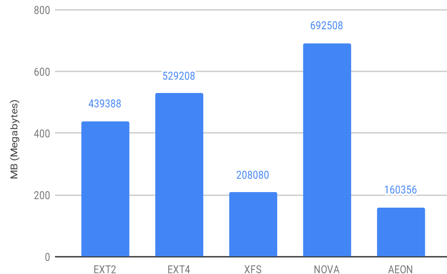
Disk Usage (less is better)
