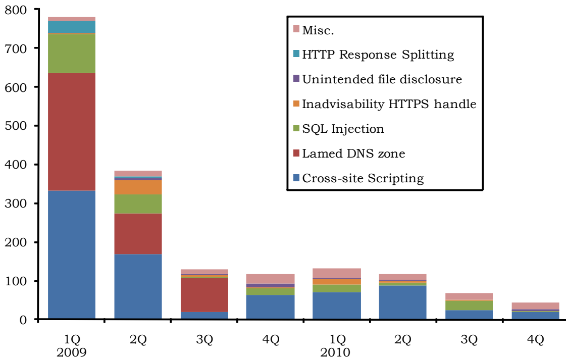
Chart 3-2: Shift in Number of Vulnerabilities in Websites by Type (from Jan 1 2009, to the End of December, 2010)
