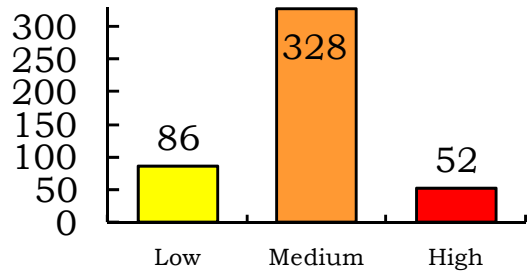
Chart 2-1 : Severity of Vulnerabilities in Software Products (from Initial Acceptance to the end of December, 2010)
