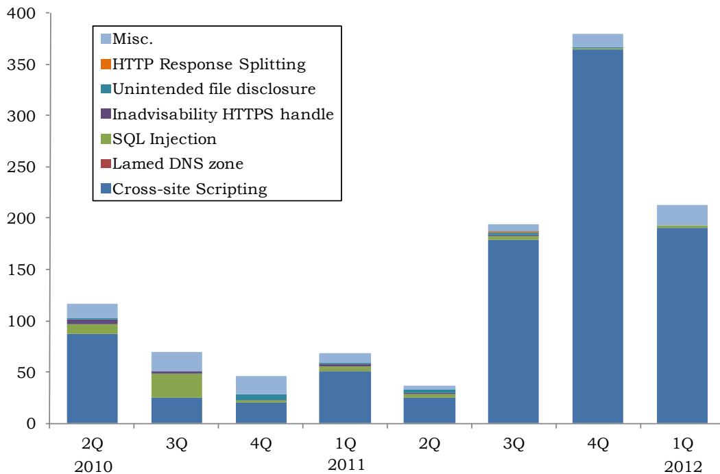
Chart 3-2: Shift in Number of Vulnerabilities in Websites by Type (from April 1 2010, to the End of March, 2012)
