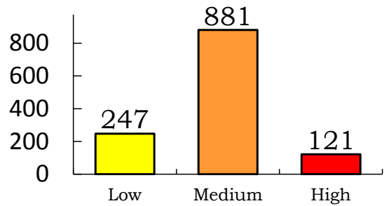
Chart 2-1 : Severity of Vulnerabilities in Software Products on JVN Several reports may be summarized in one on JVN. (from Initial Acceptance to the end of June, 2016)
