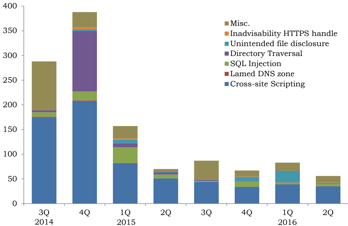
Chart 3-2: Shift in Number of Vulnerabilities in Websites by Type (from July 1 2014, to the End of June, 2016)
