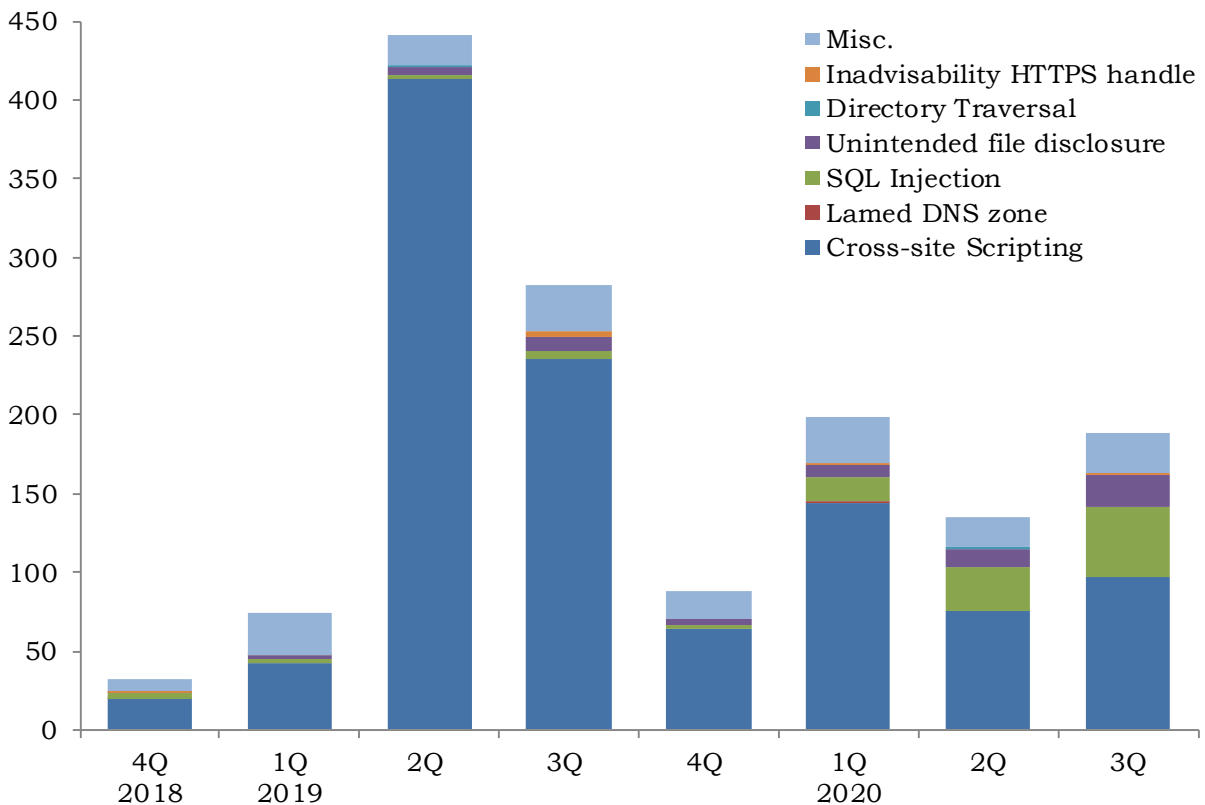
Chart 3-2: Shift in Number of Vulnerabilities in Websites by Type (from October 1 2018, to the End of September, 2020)
