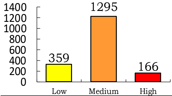
Chart 2-1 : Severity of Vulnerabilities in Software Products on JVN Several reports may be summarized in one on JVN. (from Initial Acceptance to the end of September, 2020)
