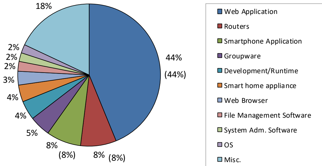
Chart 2-2: Breakdown of the Vulnerabilities in Software Products (from July 8, 2004 to the end of September, 2020)
