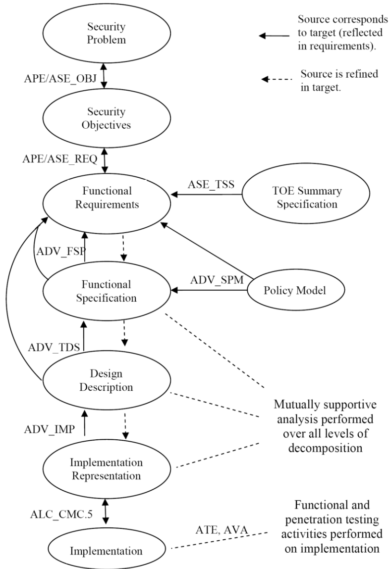
Figure 11 - Relationships of ADV constructs to one another and to other families
