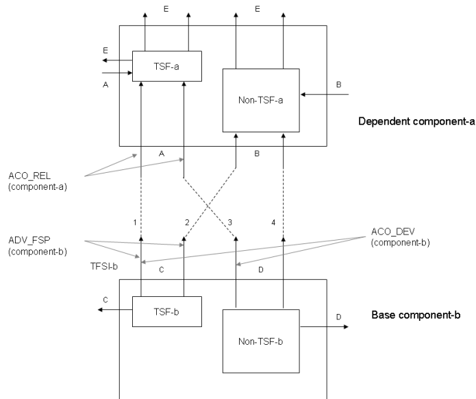
Figure 26 - Composed component interfaces
