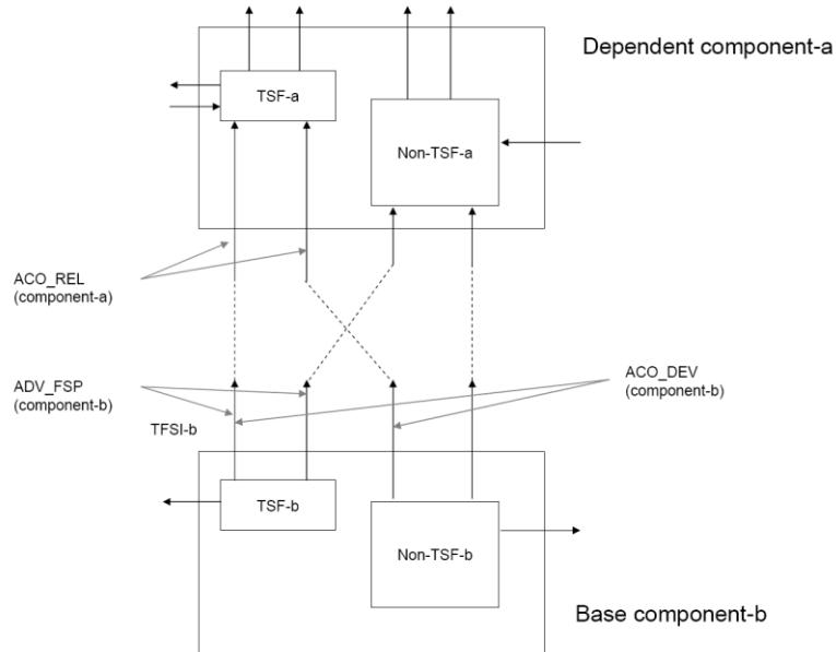
Figure 17 - Relationship between ACO families and interactions between components
